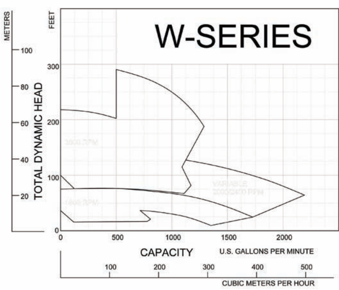
DOUBLE VOLUTE
