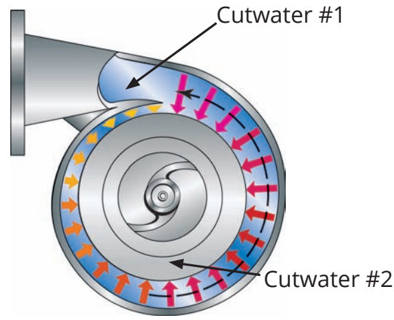
DOUBLE VOLUTE
